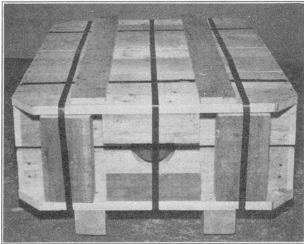
FIG. 227. Pallet-type box with skids.
