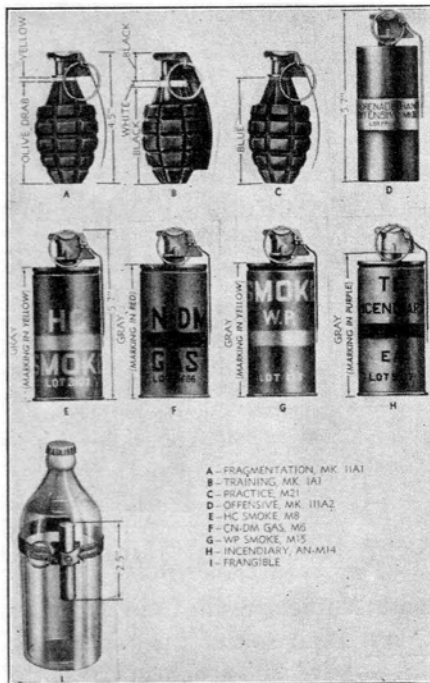
FIG. 204. Typical hand grenades.
