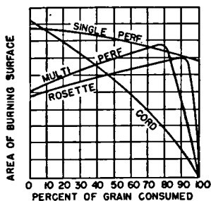
EFFECT OF GRAIN SHAPE ON BURNING RATE
