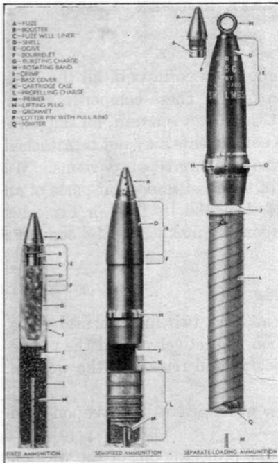
FIG. 83. Fixed, semifixed, and separate-loaded artillery rounds.
