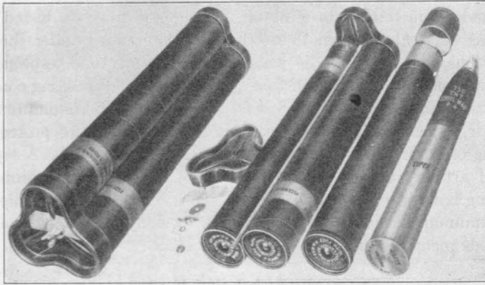
FIG. 232. Cloverleaf packing for complete rounds.
