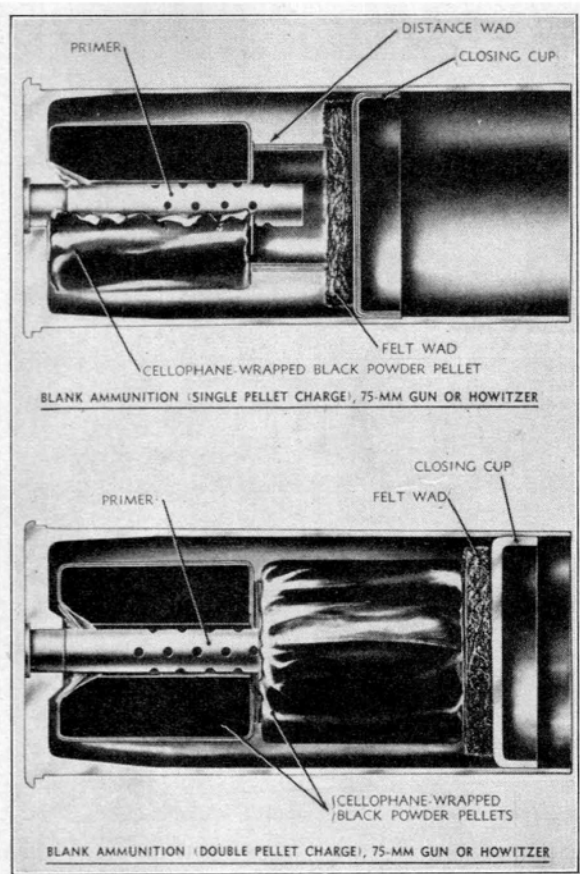
FIG. 48. Artillery blank ammunition.
