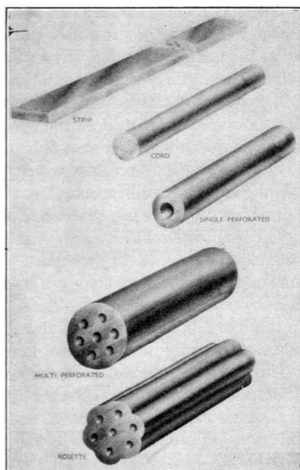
FIG. 4. Typical powder grains.
