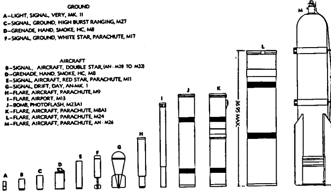
Fig. 161. Comparison of various pyrotechnics.
