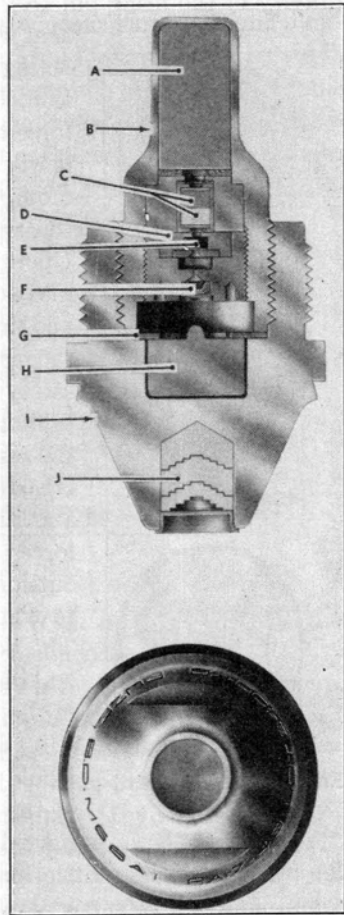
FIG. 58. M66 artillery fuze.
