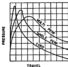
PRESSURE-DISTANCE CURVES FOR VARIOUS GRAIN SHAPES.
