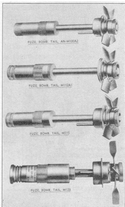
FIG. 148. Various tail bomb fuzes.
