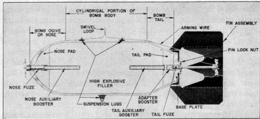
FIG. 103. Components of bomb complete round.
