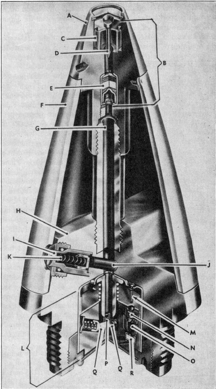
FIG. 68. M48A2 artillery fuze. 153
