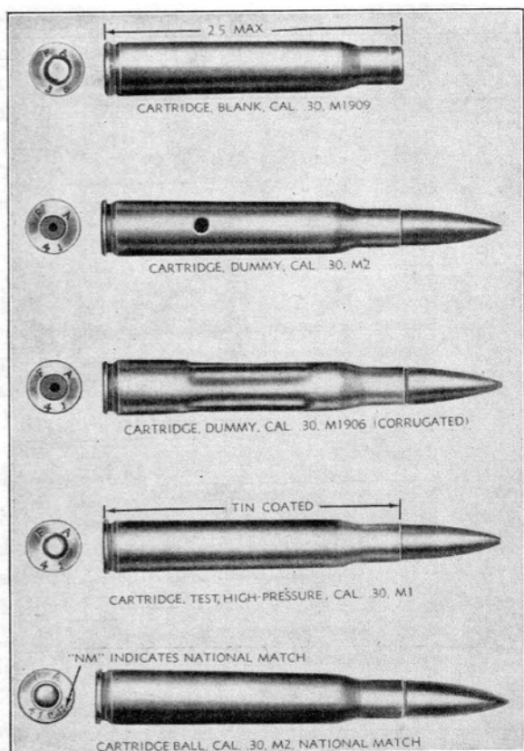
FIG. 35. Caliber .30 cartridges.
