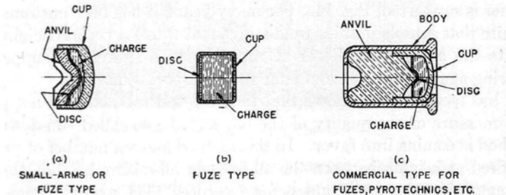
FIG. 13. Typical fuze-type primers.
