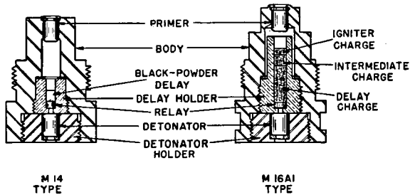
FIG. 150. Details of primer detonators.
