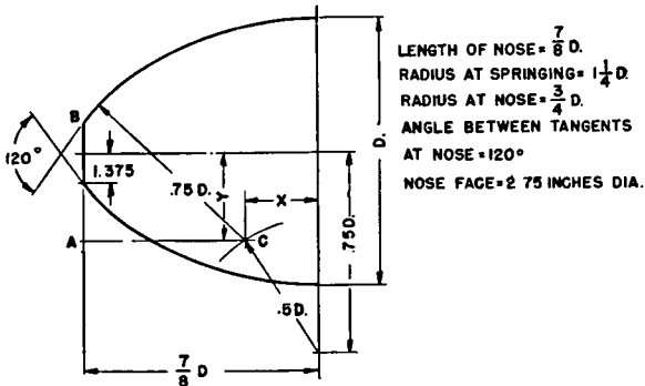
FIG. 101. Bomb-nose design.
