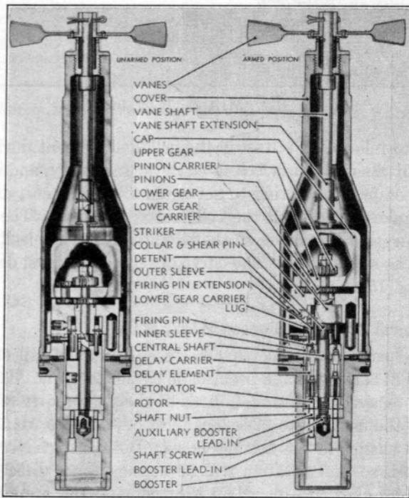
FIG. 157. Mk 228 tail bomb fuze.
