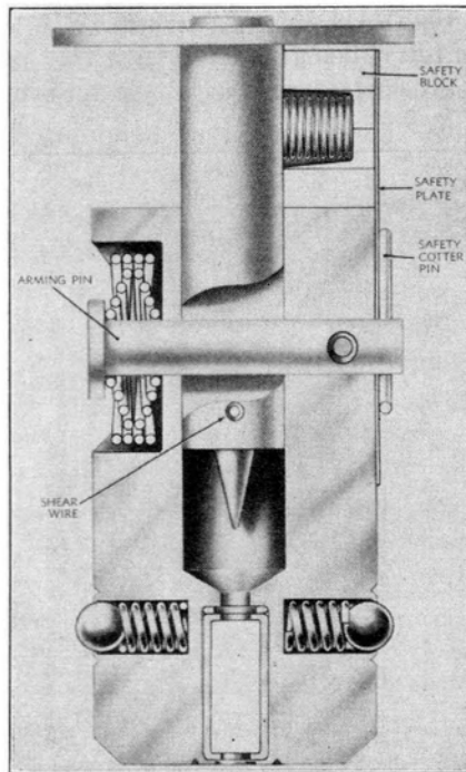
FIG. 142. M108 nose bomb fuze.
