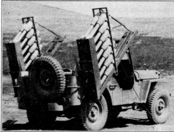
FIG. 200. Launcher mounted on \frac{1}{4} -ton truck
