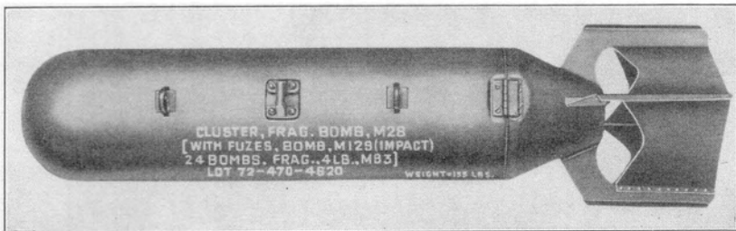
FIG. 122. Cluster of twenty-four 4-lb. butterfly bombs (adapter closed).
