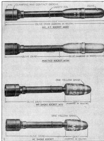
FIG. 193. 2.36-in. rockets.
