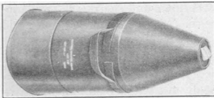
FIG. 223. M2A3 10-lb. shaped-charge demolition block.
