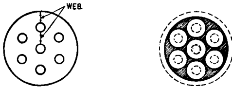
FIG. 6. Web and slivers of propellant powder grains. (Dotted lines show original grain size.)
