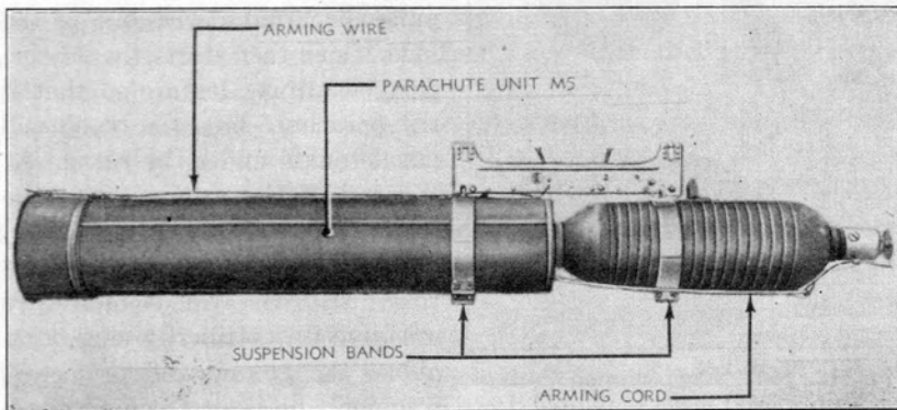
FIG. 111. 90-lb. fragmentation bomb with parachute.
