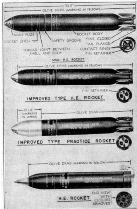
FIG. 195. 4.5-in. rockets.
