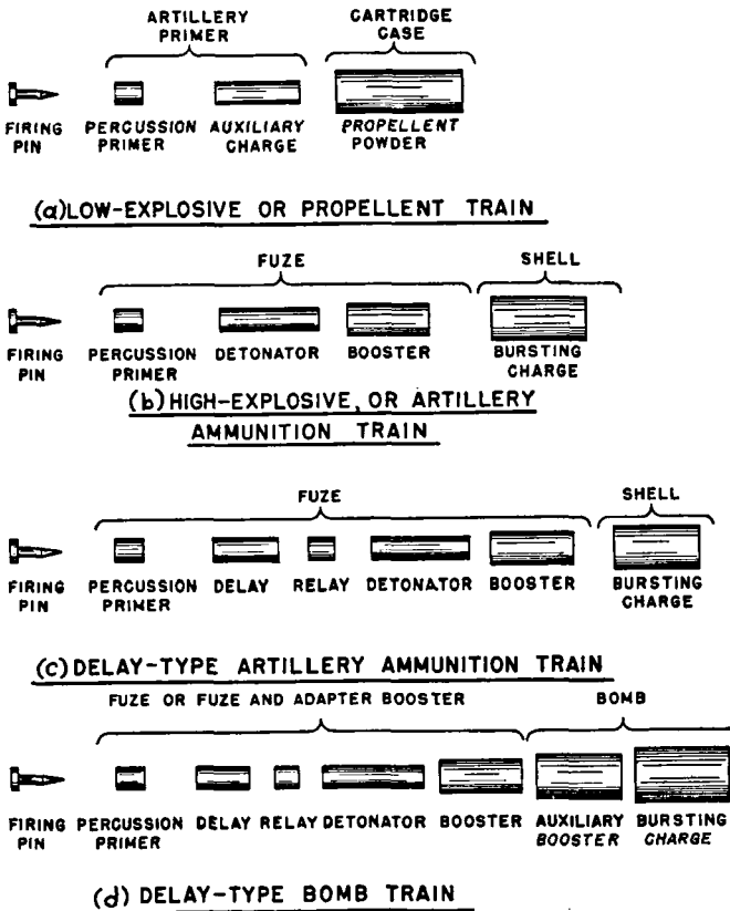
FIG. 3. Diagram of elements of explosive trains.
