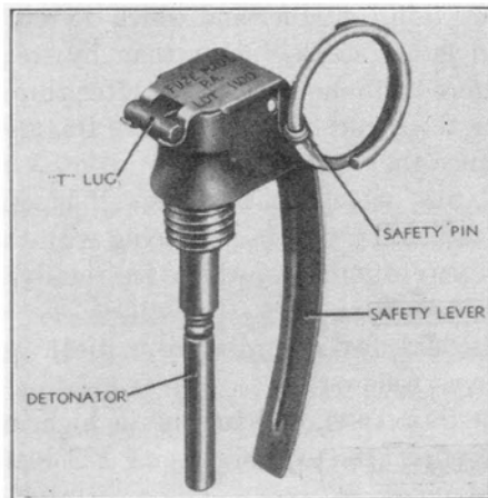
FIG. 202. Typical hand-grenade fuze.
