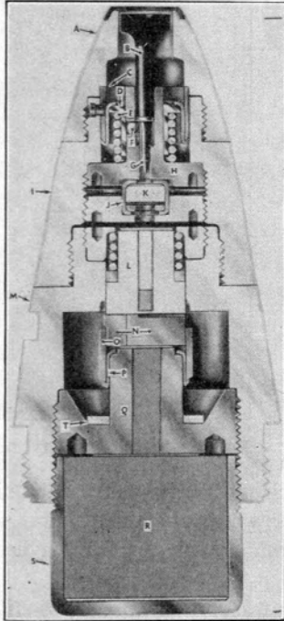
FIG. 64. No. 251 artillery fuze.
