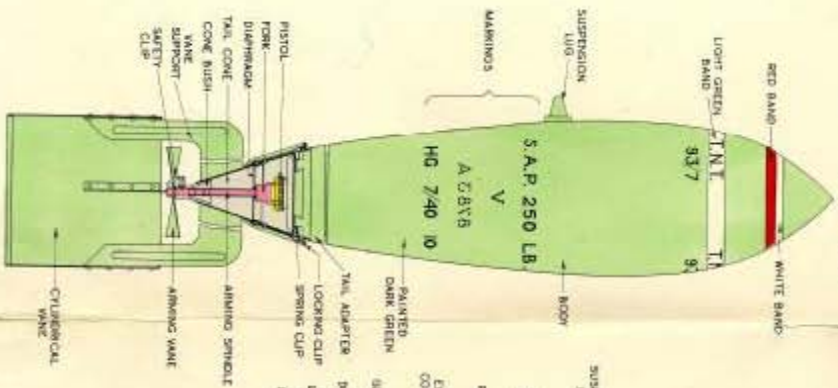
BOMB HE S.A.P. 250LB MARK V
