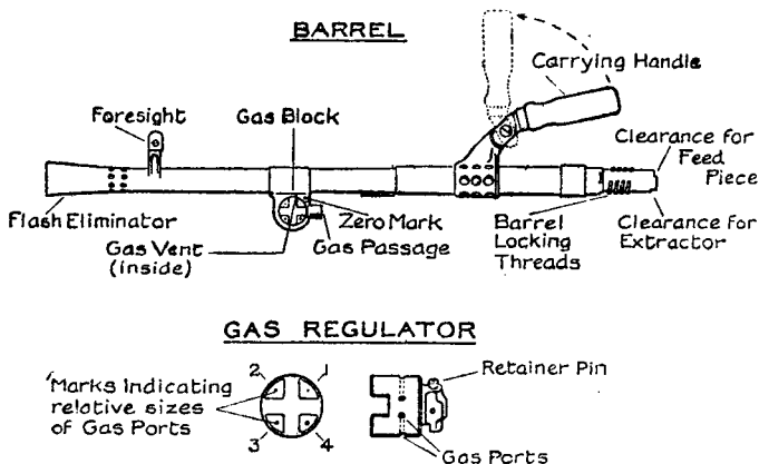
FIG. 7.—Barrel Group.
