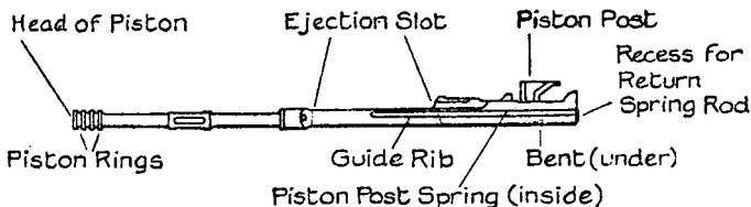
FIG. 6.—Piston Group.
