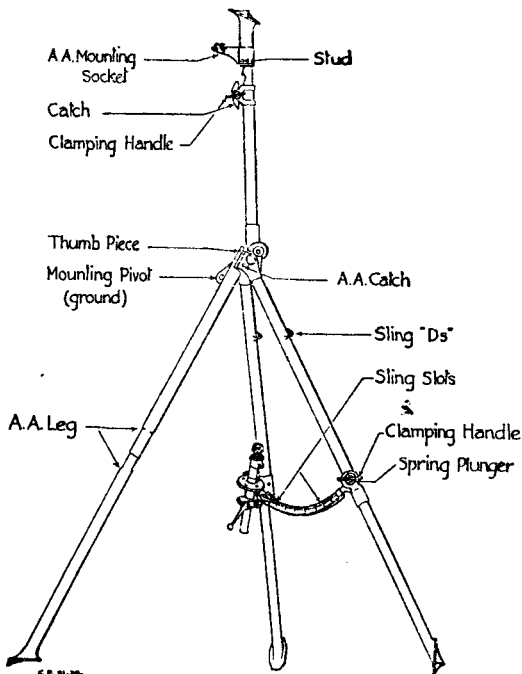
FIG. 12.—The Tripod, Anti-Aircraft.
