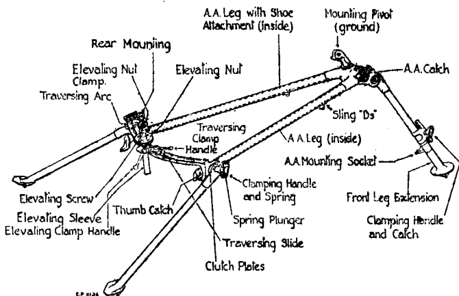
FIG. 11.—The Tripod (Ground).
