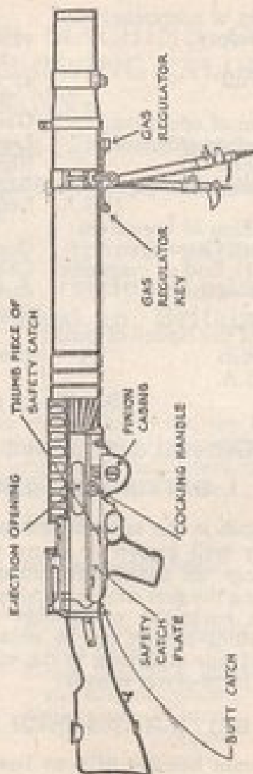
LEWIS LIGHT MACHINE GUN
