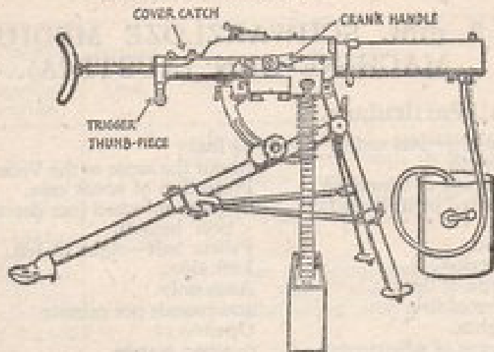
Schwarzloze Medium Machine Gun.
