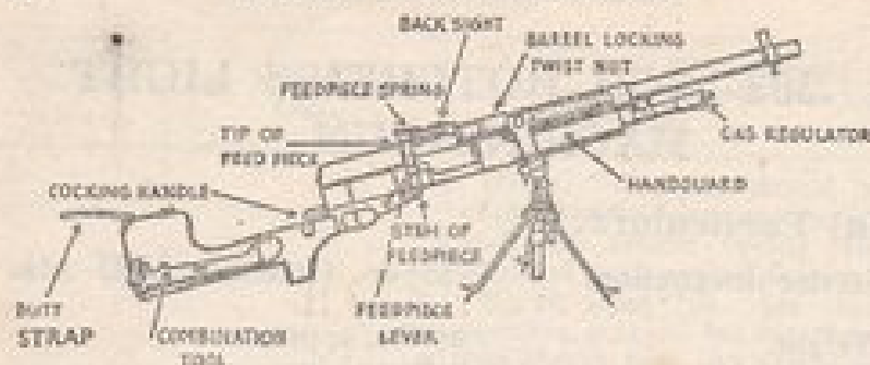
HOTCHKISS LIGHT MACHINE GUN
