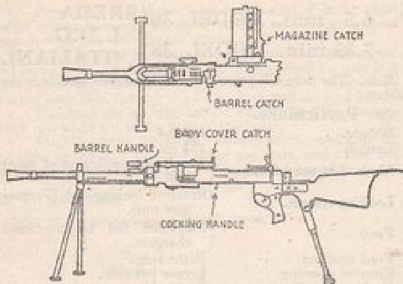
BREDA L.M.G. 6.5 MM. MODEL '30.
