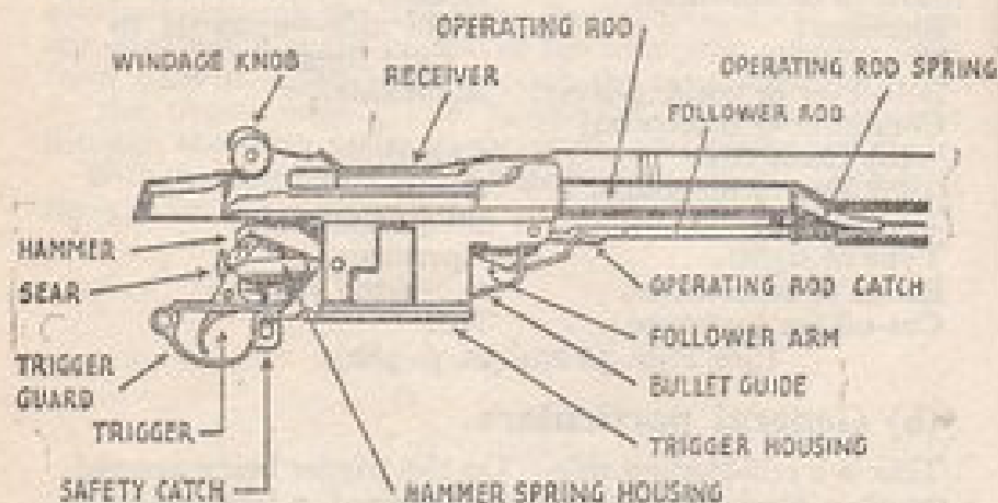
RIGHT SIDE OF .300 GARAND
