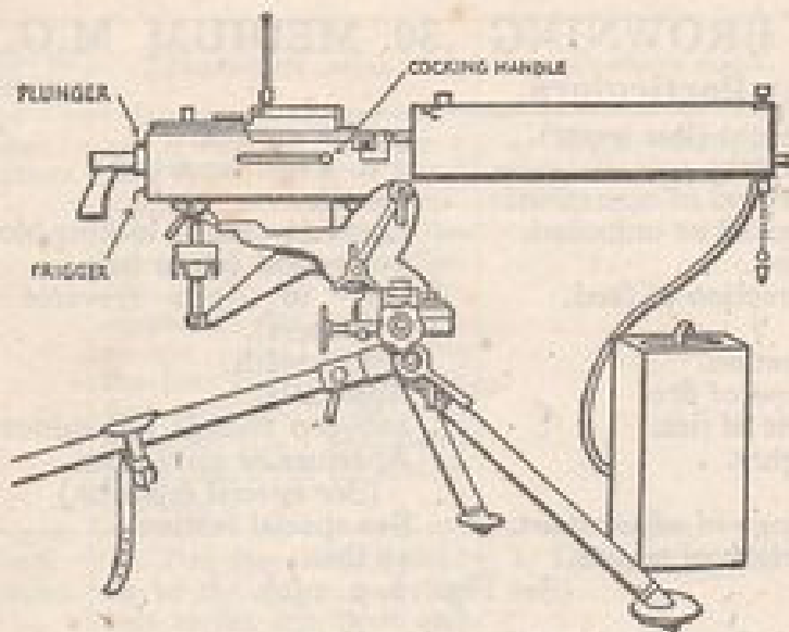
BROWNING MEDIUM MACHINE GUN
