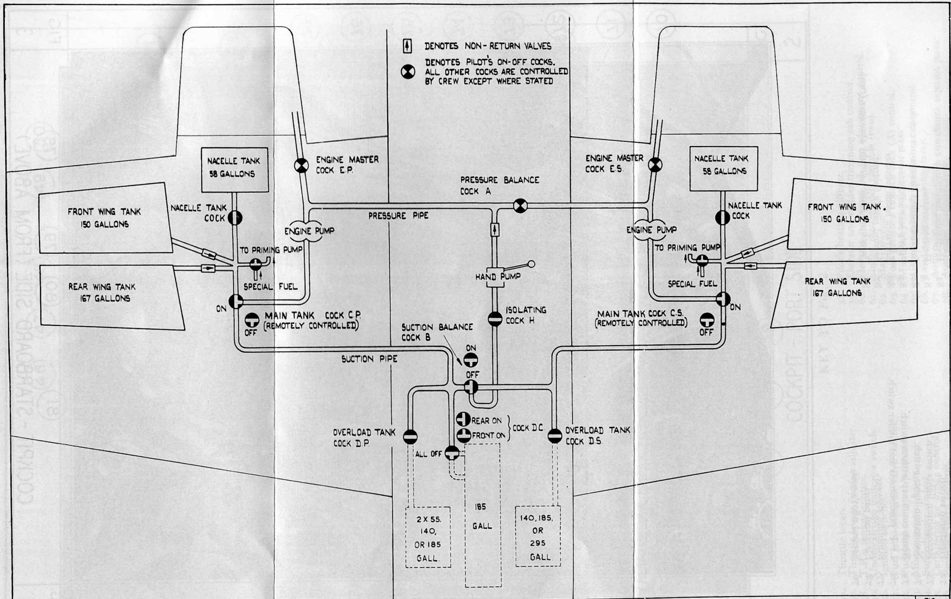
FUEL SYSTEM DIAGRAM
